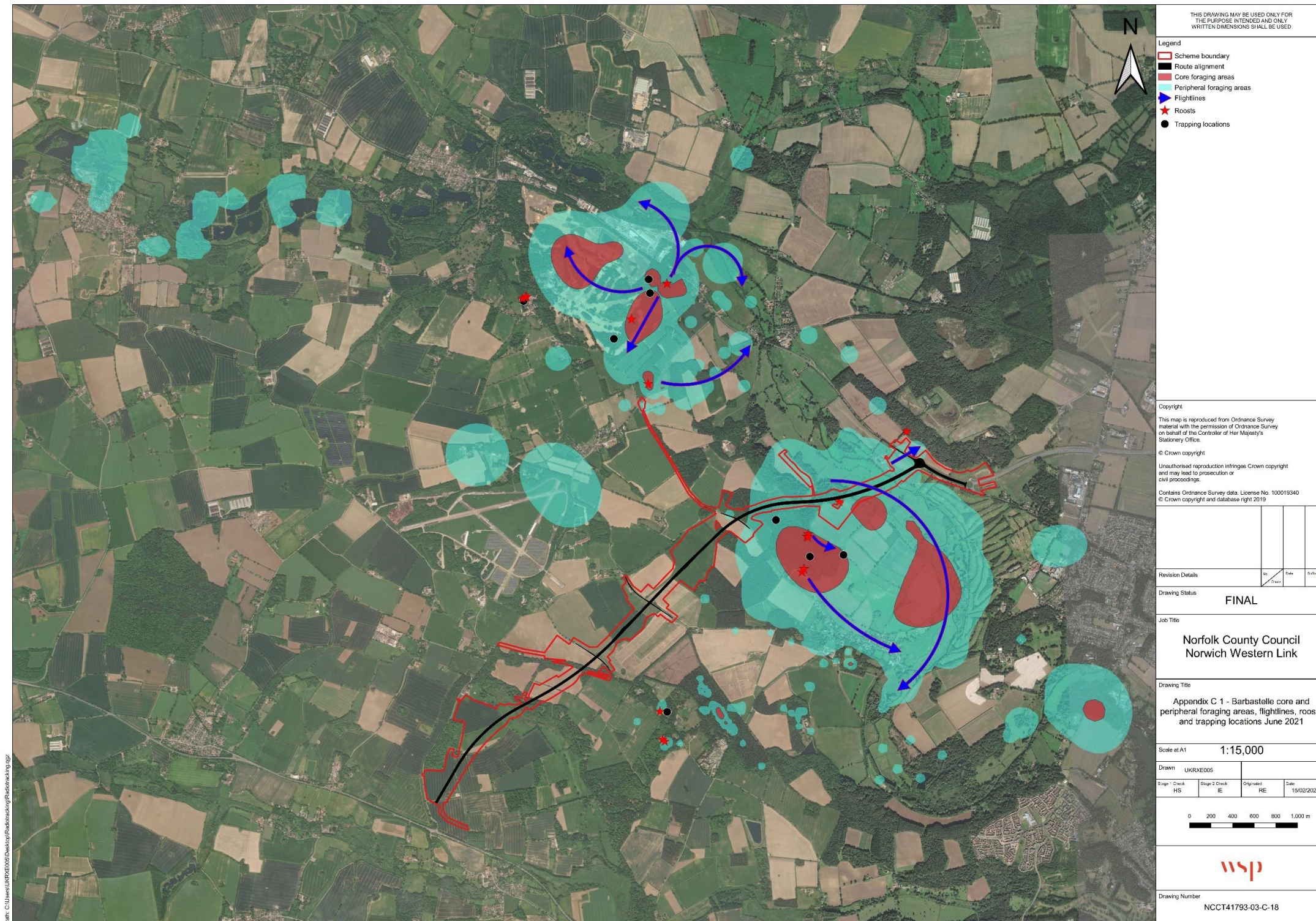
Figure C1 – Barbastelle core and peripheral foraging areas, flight lines, roosts and trapping locations June 2021
